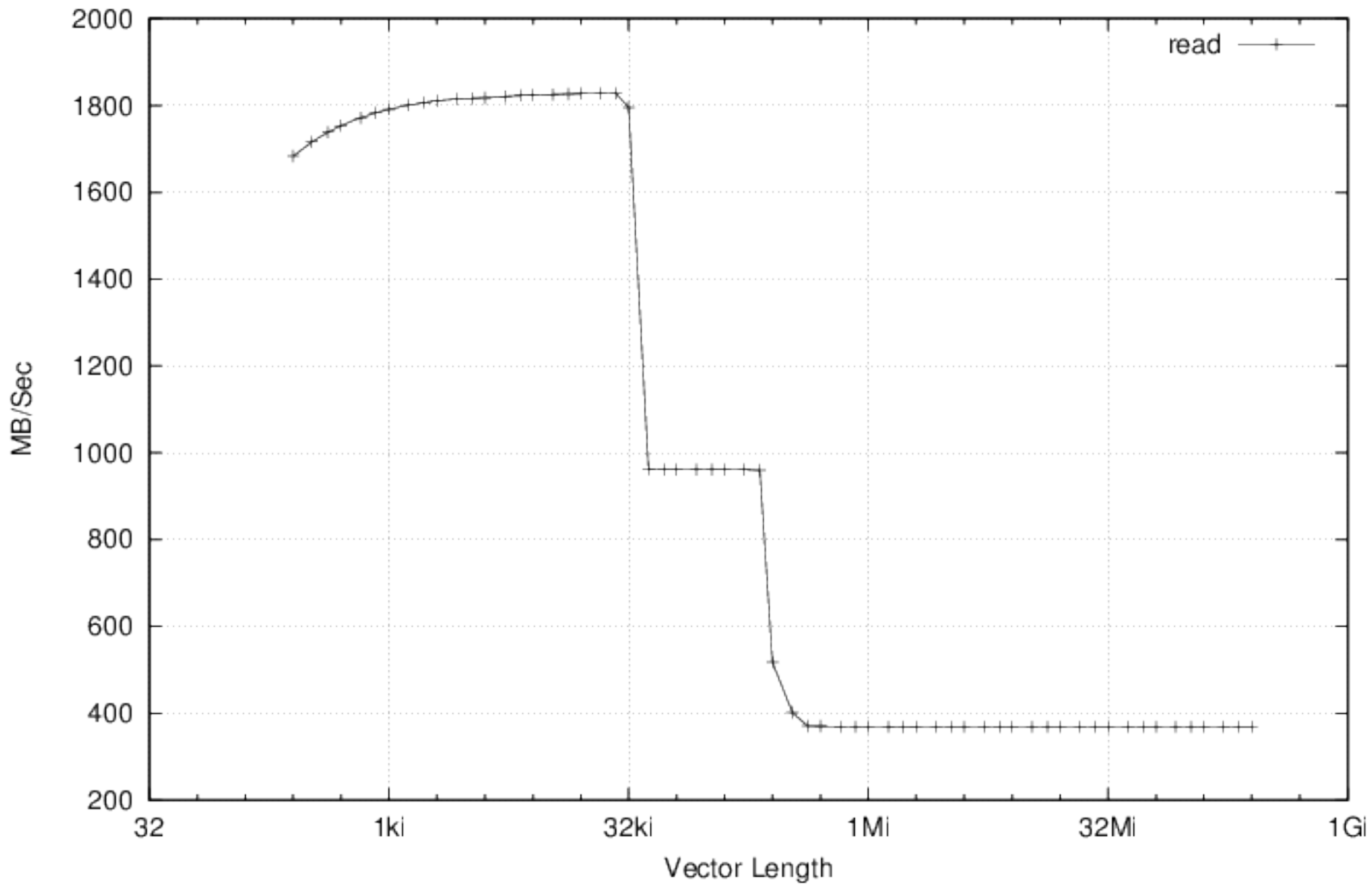
Non official Cachebench results on the mainline Linux port ( kernel 3.6-rc2 ) of Armada 370 with L2Cache support
