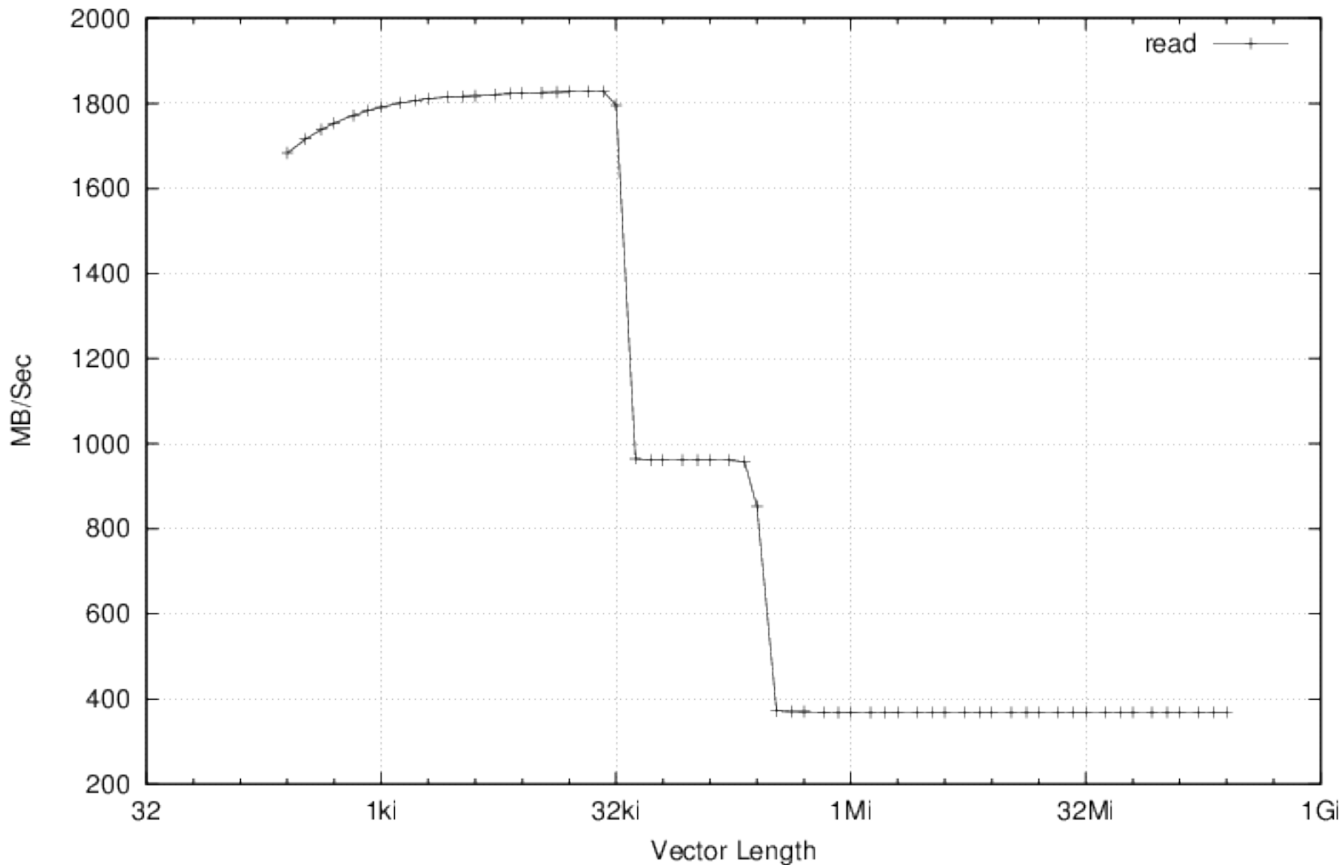
Non official Cachebench results on the mainline Linux port ( kernel 3.6-rc4 ) of Armada 370 with L2Cache support
