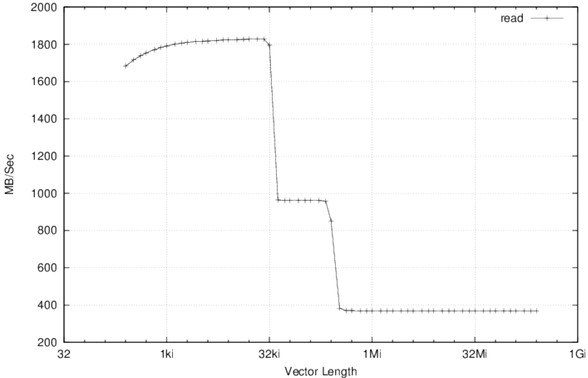
Non official Cachebench results on the mainline Linux port ( kernel 3.6rc1 ) of Armada 370 with L2Cache support
