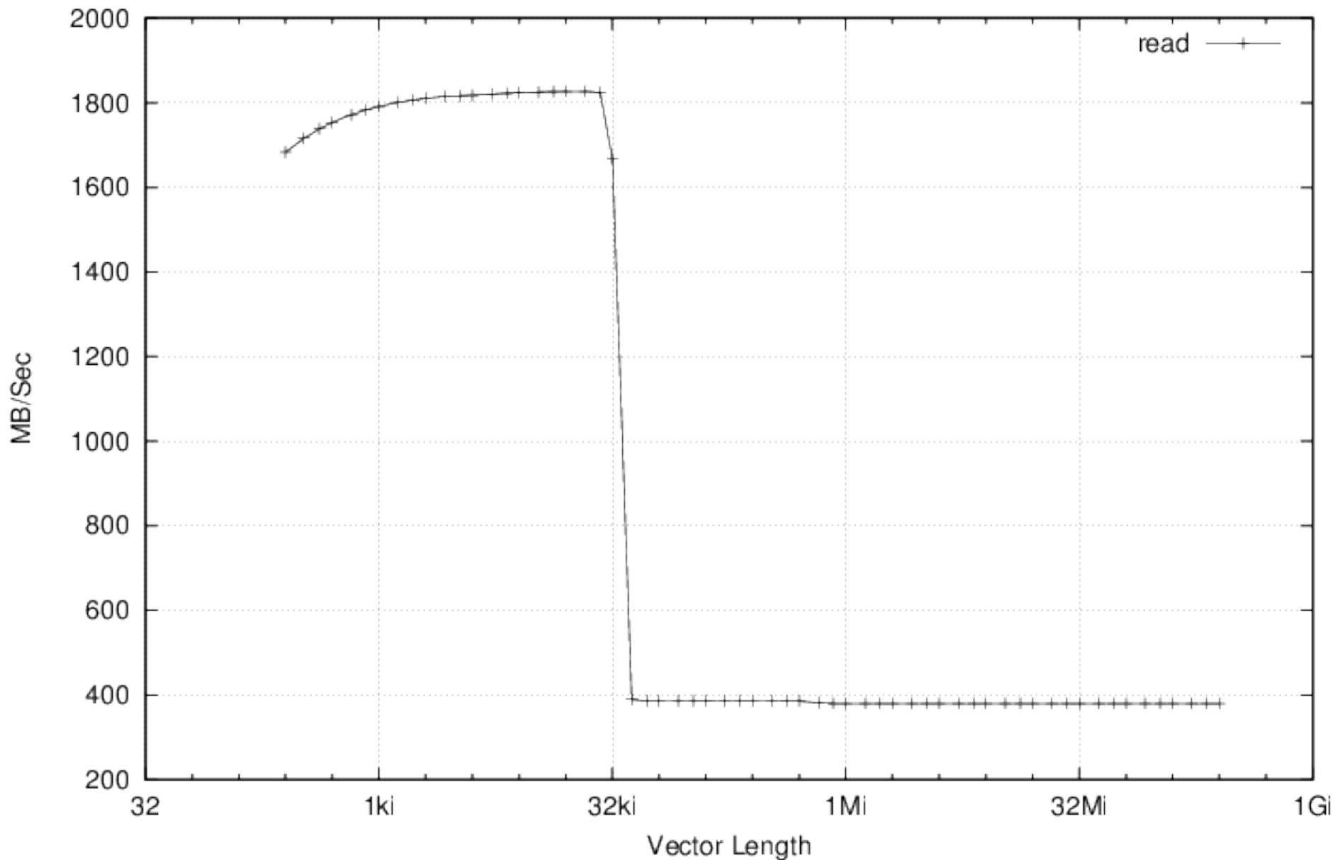
Non official Cachebench results on the mainline Linux port ( kernel 3.6-rc2 ) of Armada 370 without L2Cache support
