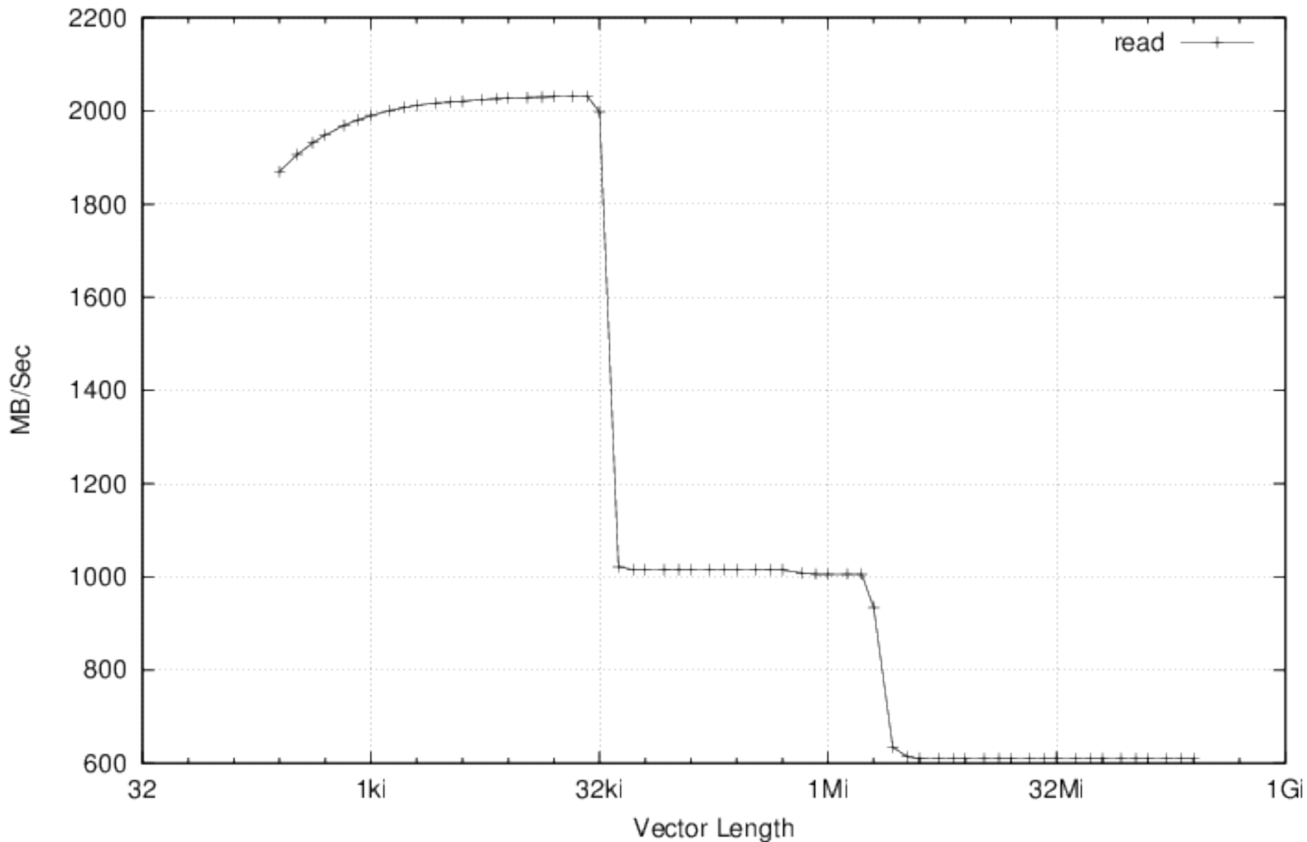
Non official Cachebench results on the mainline Linux port ( kernel 3.6-rc2 ) of Armada XP with L2Cache support
