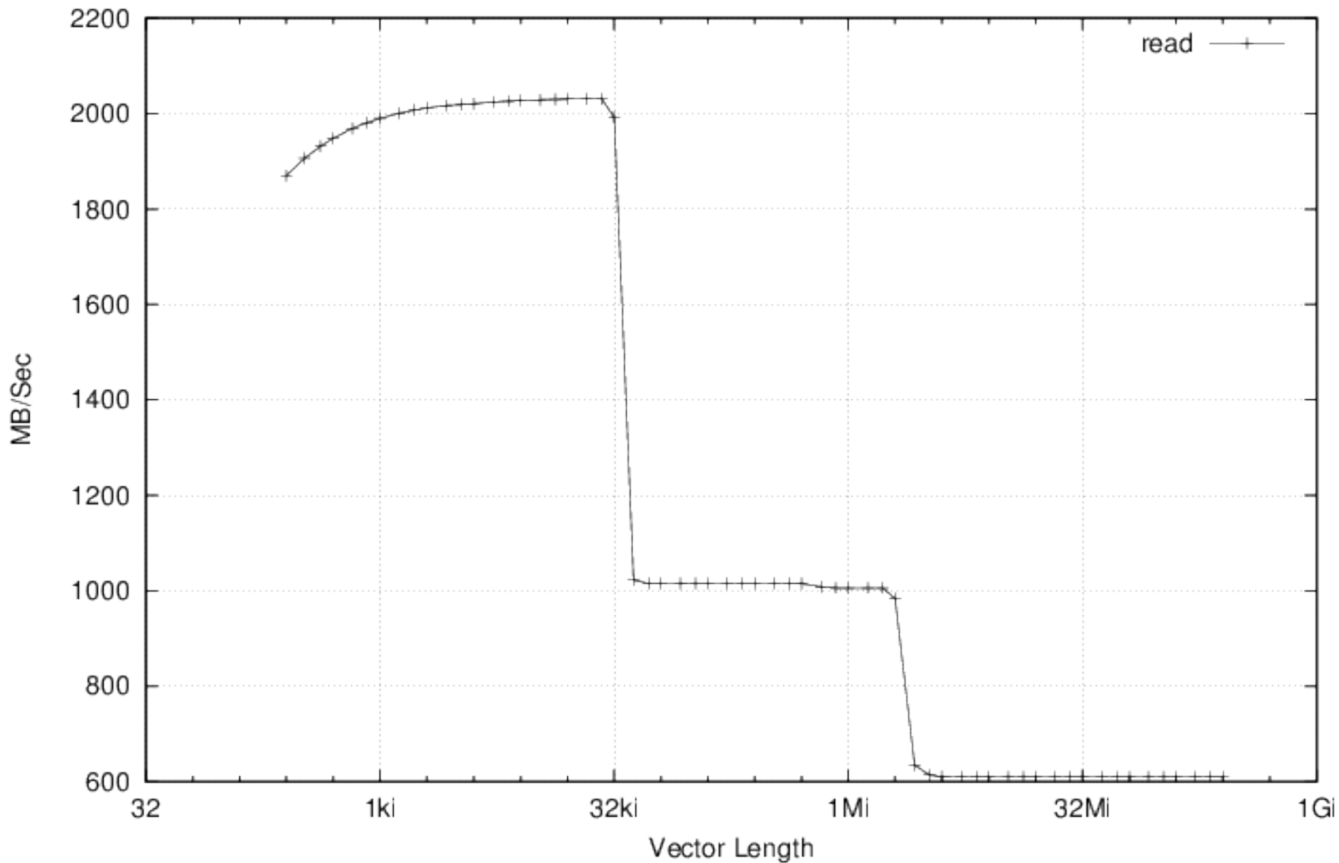
Non official Cachebench results on the mainline Linux port ( kernel 3.6-rc4 ) of Armada XP with L2Cache support
