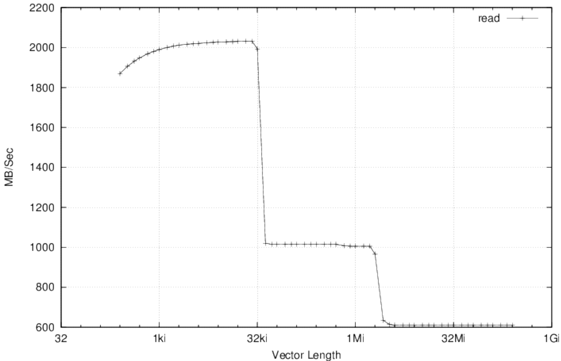
Non official Cachebench results on the mainline Linux port ( kernel 3.6rc1 ) of Armada XP with L2Cache support
