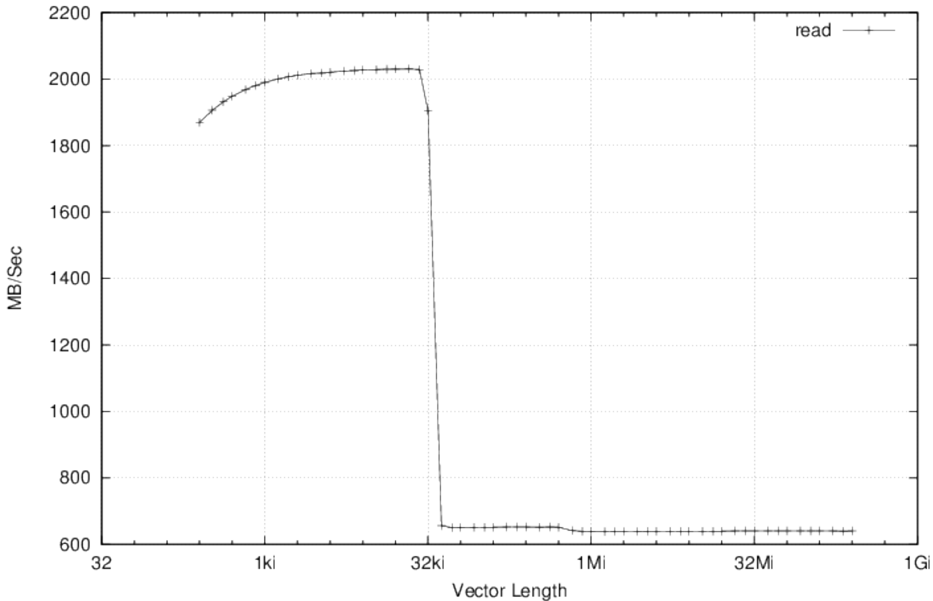
Non official Cachebench results on the mainline Linux port ( kernel 3.6-rc2 ) of Armada XP without L2Cache support
