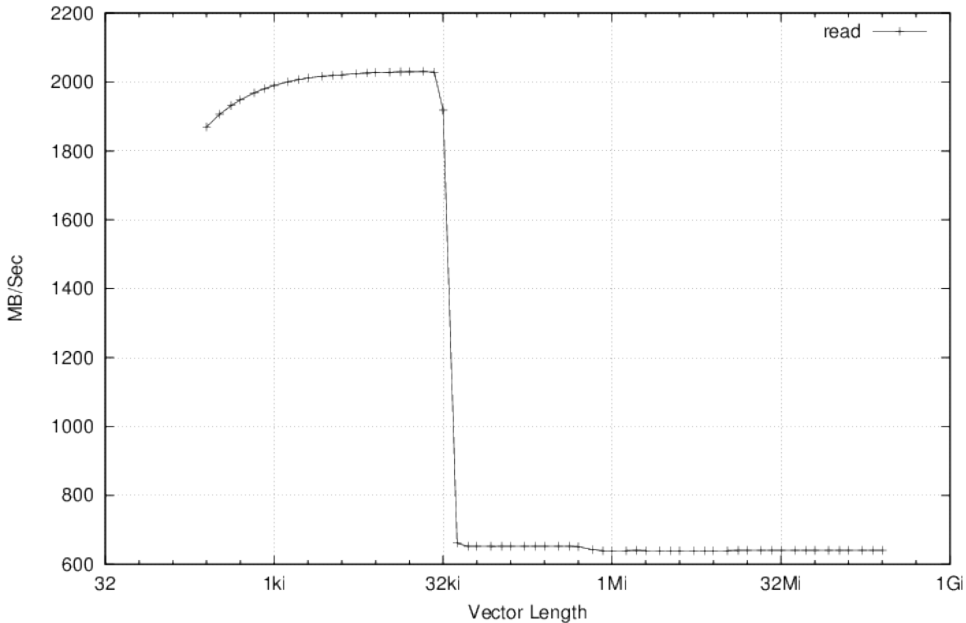
Non official Cachebench results on the mainline Linux port ( kernel 3.6rc1 ) of Armada XP with No L2Cache support
