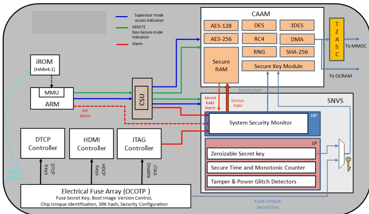
Figure 11-1. Security subsystem (simplified)
