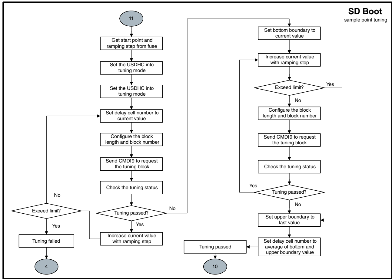
Figure 8-16. Expansion Device Boot Flow (6 of 6) i.MX 6Dual/6Quad Applications Processor Reference Manual, Rev. 2, 06/2014
