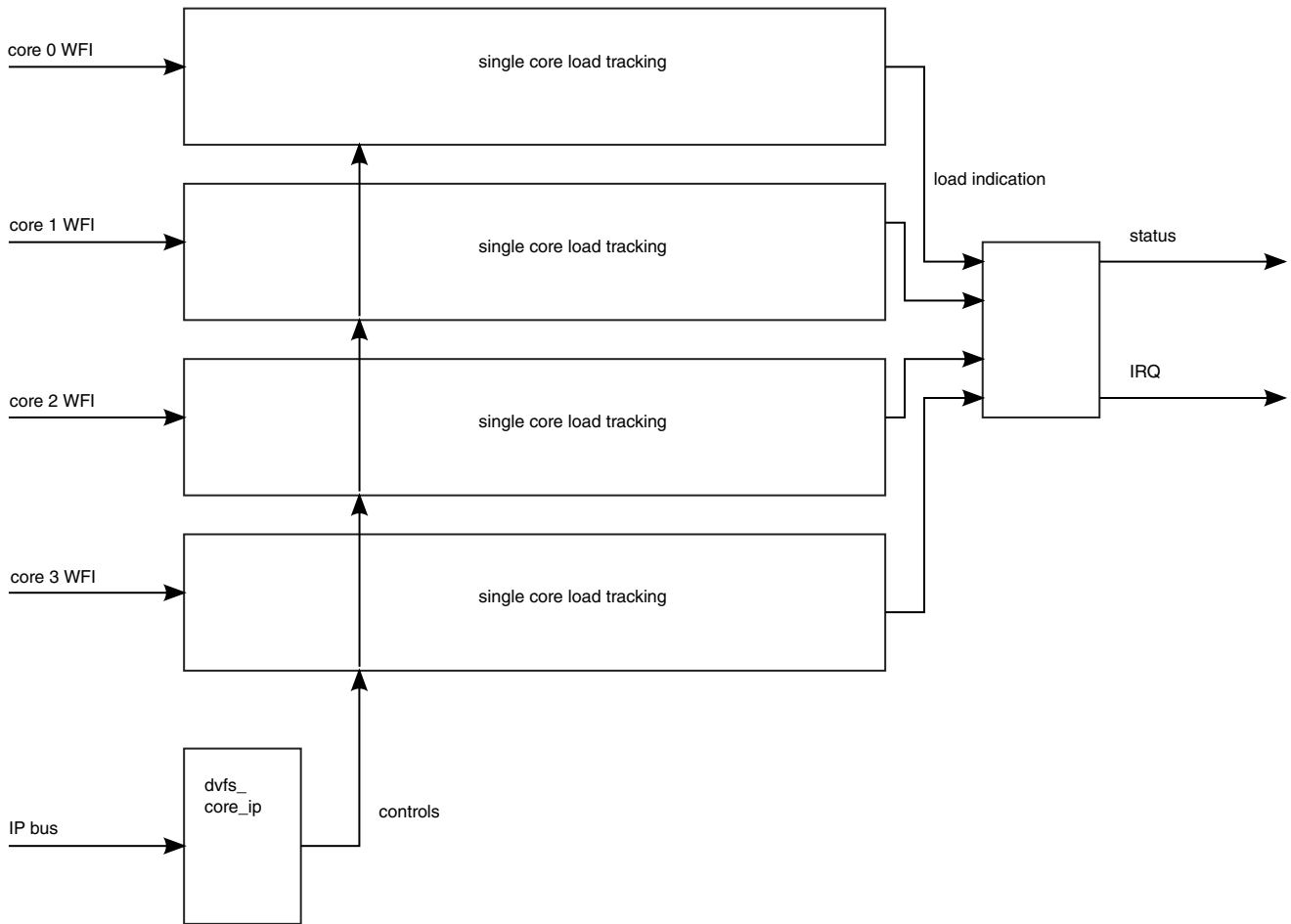
Figure 27-2. DVFS_core diagram
