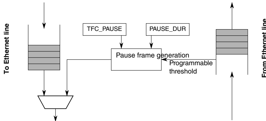
Figure 23-108. Pause frame generation overview
