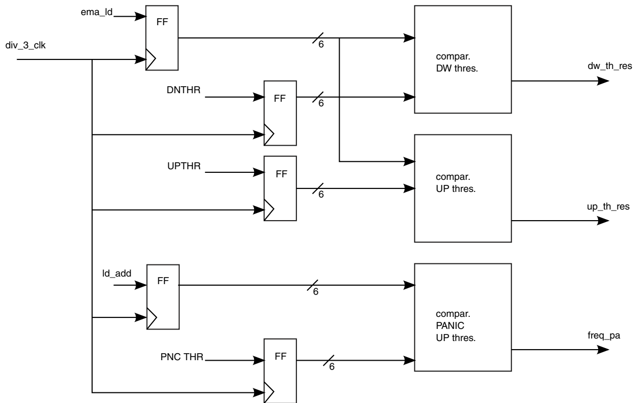
Figure 27-10. dvfs_tresh_cmp diagram
