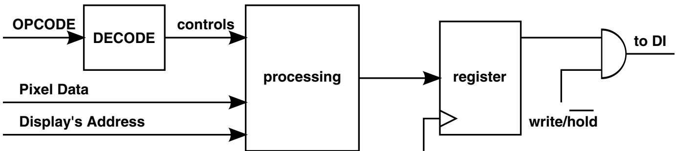
Figure 37-31. Opcode processing
