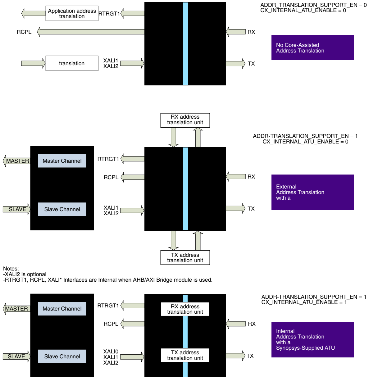
Figure 48-24. Address Translation options
