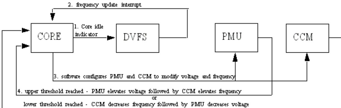
Figure 10-11. High Level DVFS working flow
