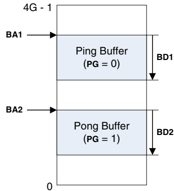
Figure 43-7. Ping-Pong System Memory Structure
