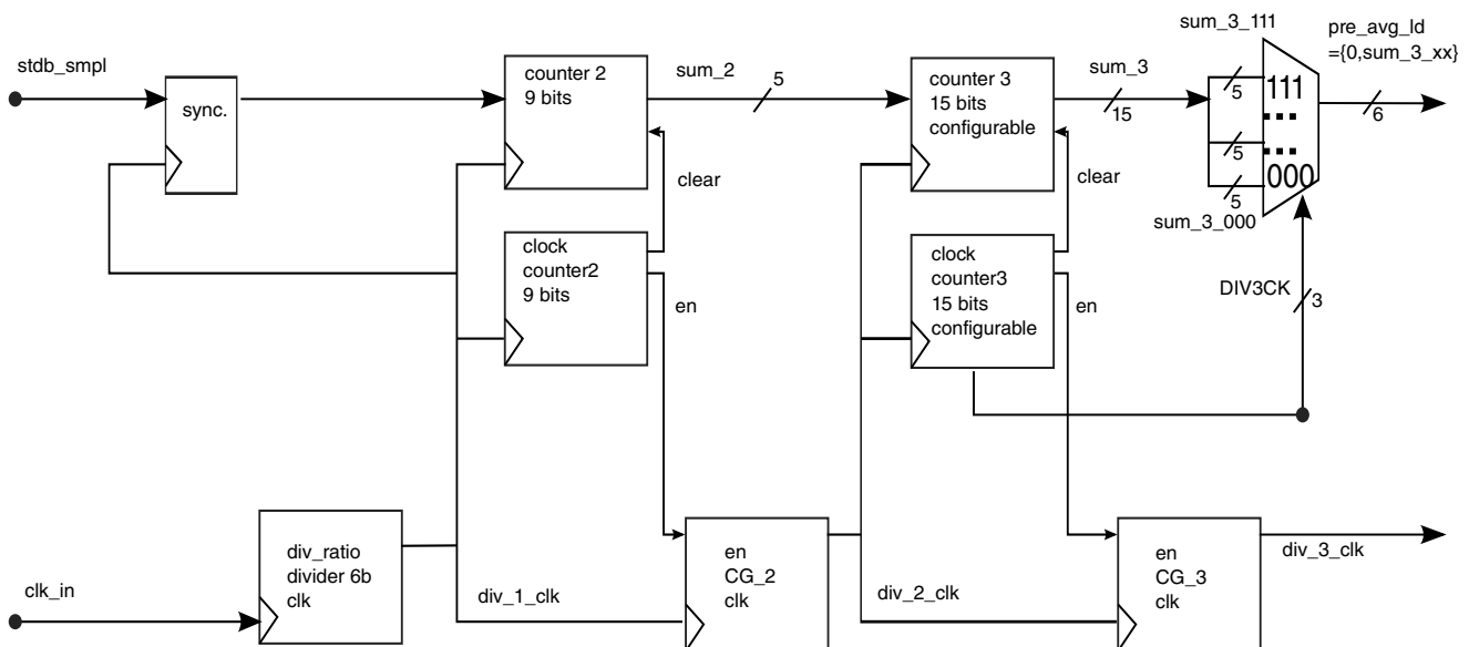
Figure 27-6. dvfs_pre_avg block diagram
