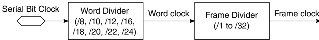
Figure 61-21. SSI Clocking
