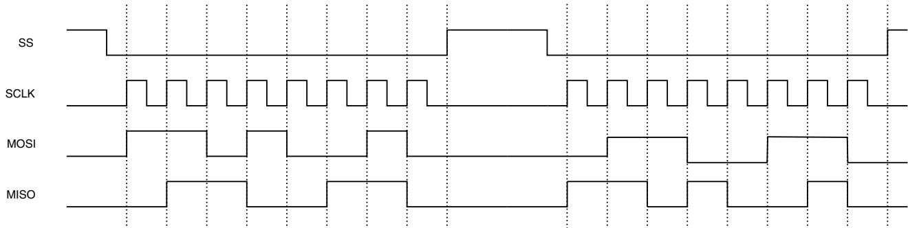
Figure 21-9. SPI Bursts While SS\_CTL[3:0] is Set
